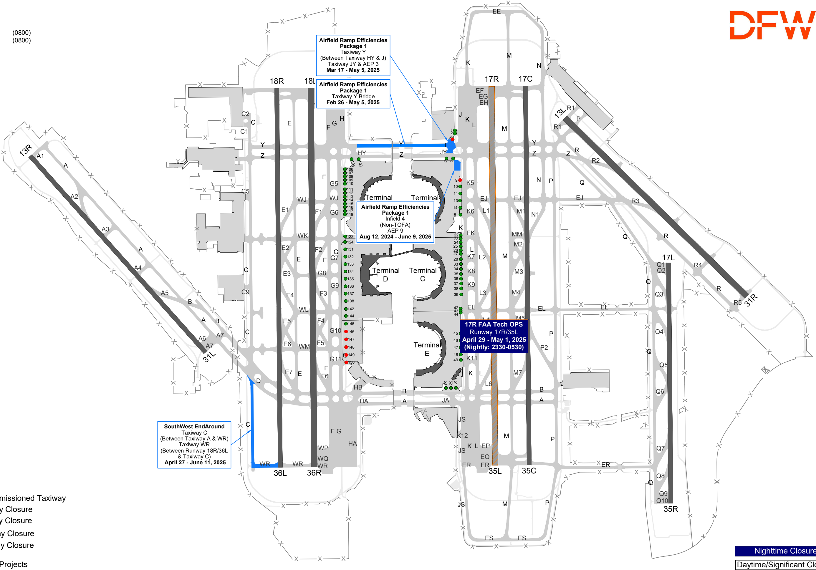
Airfield Short-Term Operational Phasing: Sunday April 27, 2025 - Saturday May 3, 2025
